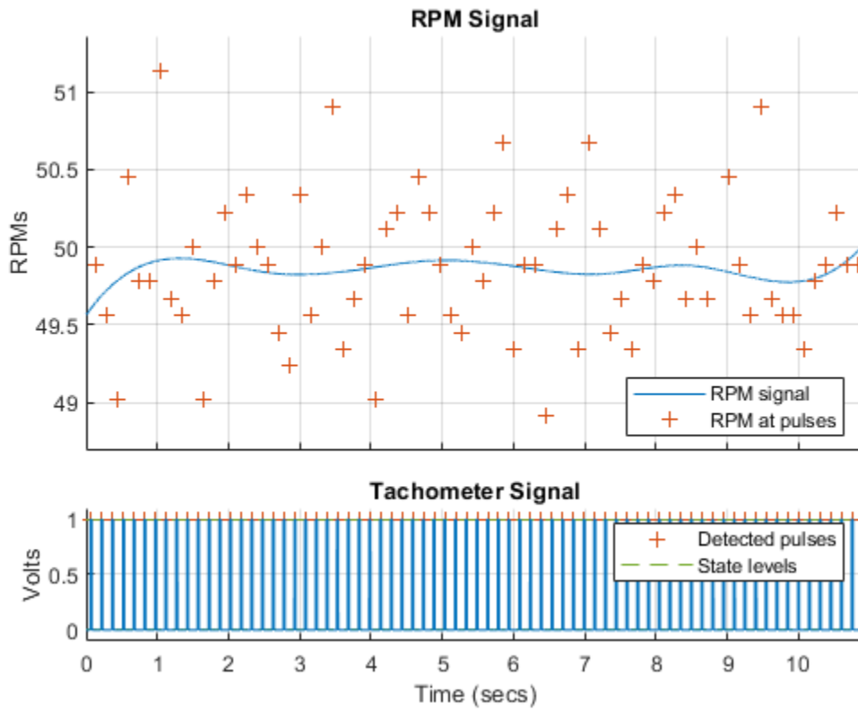
figure tachorpm(faultyTacho,fs, 'PulsesPerRev',8)
